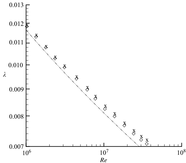
FIGURE 1. Data with new static pressure and Pitot corrections, \diamond , compared with Prandtl's friction factor relationship (---) and the ZS friction factor data ( \times ).
